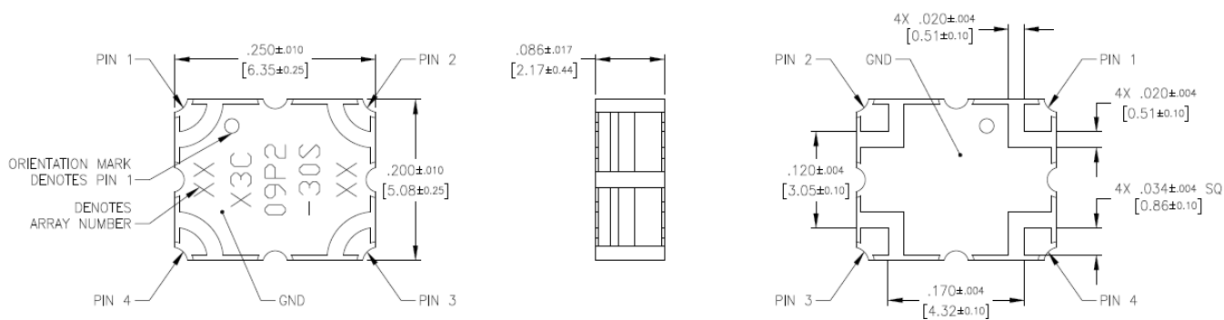
Dimensions are in Inches [Millimeters] X3C09P2-30S Mechanical Outline
