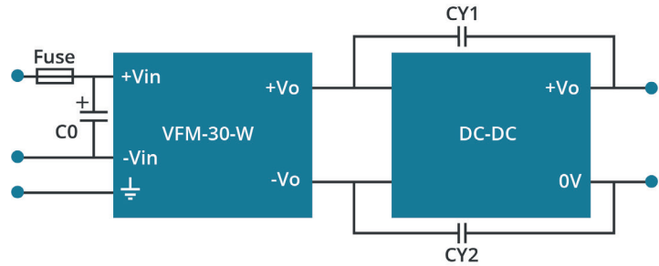
Figure 1 Application Circuit
