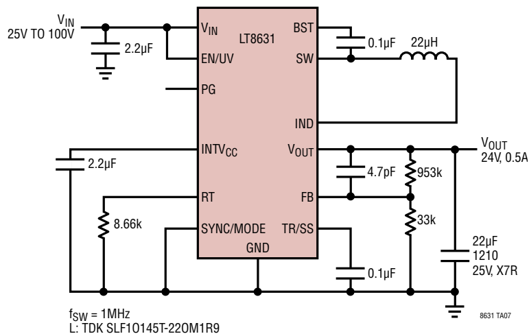
1MHz, 24V, 0.5A Step-Down Converter
