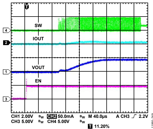
Figure 4. Buck1 Startup, V_{OUT1} = 1.8\text{ V} , I_{OUT1} = 5\text{ mA}
