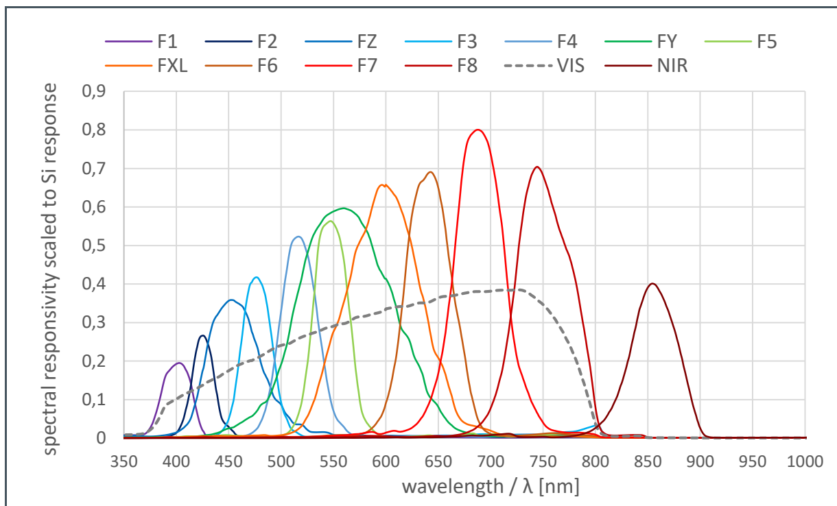
Figure 11: Spectral Responsivity
