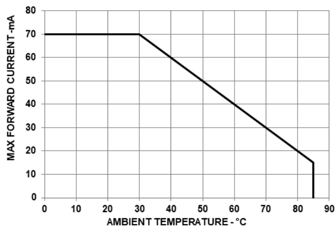
Figure 5: Derating Curve
