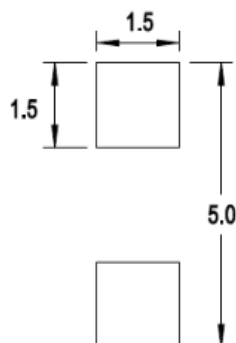
Figure 6: Recommended Soldering Land Pattern
