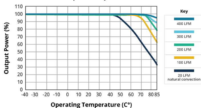
TEMPERATURE DERATING CURVE PRQ150W-Q48-S24-H-D (Heatsink version) ( V_{in} = 24\text{ V} )
