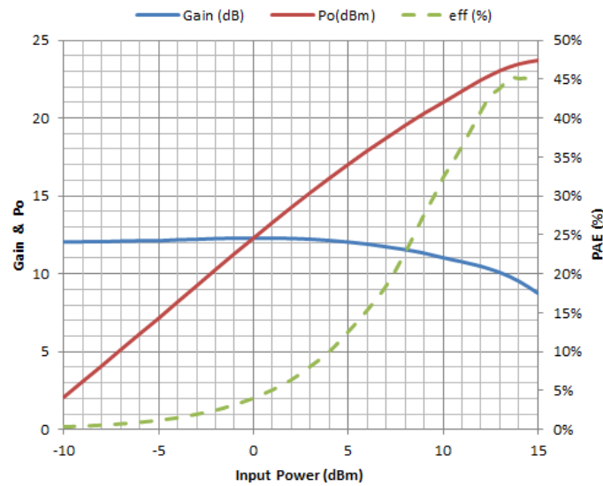
MwT-PH33F, Po, Gain & PAE vs Pin at 18GHz V_{ds}=8V ; I_{dq}=0.7 \times I_{DSS}
