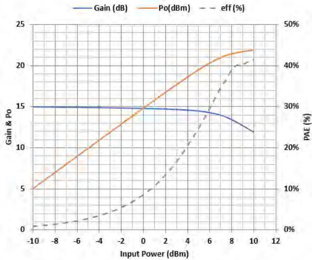
MwT-5F, Typical Power, 12GHz Vds=7V; Ids=0.6xIDSS; Vgs2=1.5V
