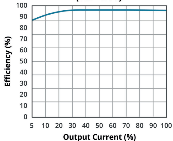
EFFICIENCY VS OUTPUT LOAD VX78015-500-W (Vin = 24 V)
