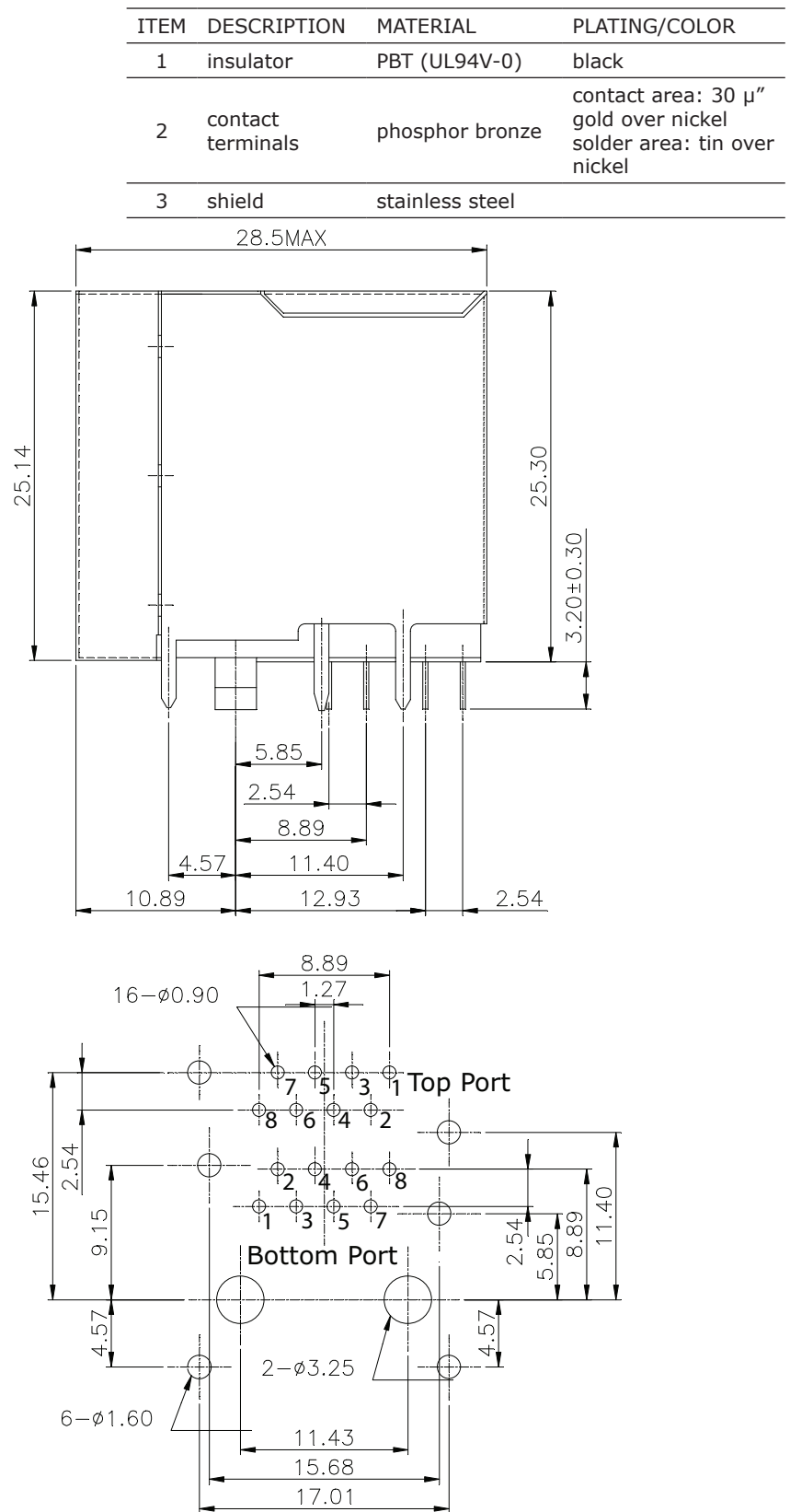
Recommended PCB Layout Top View
