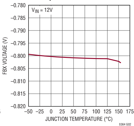
FBX Negative Regulation Voltage vs Temperature
