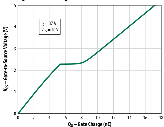
Figure 7: Gate Charge
