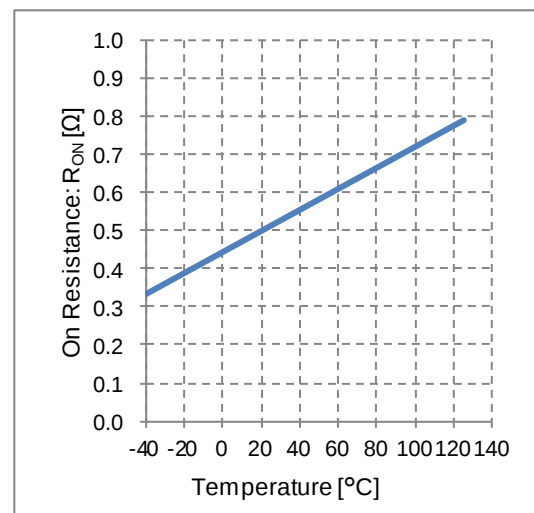
Figure 19. On Resistance vs Temperature
