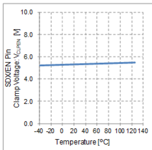
Figure 13. SDX/EN Pin Clamp Voltage vs Temperature
