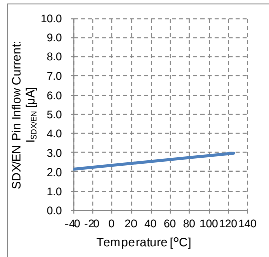
Figure 17. SDX/EN Pin Inflow Current vs Temperature
