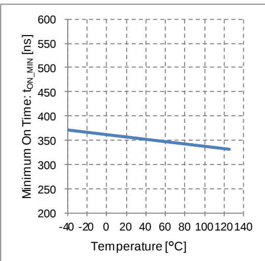
Figure 23. Minimum On Time vs Temperature
