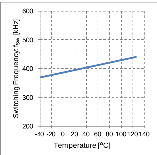
Figure 21. Switching Frequency vs Temperature
