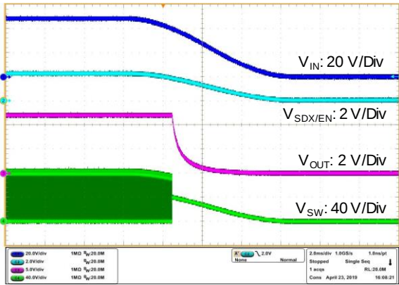
Figure 41. Shutdown Waveform (The VIN Pin Control)
