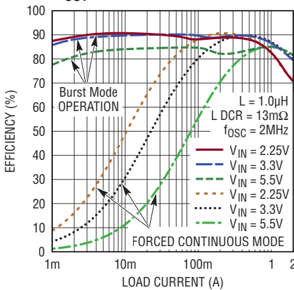
2A Buck Efficiency vs I_{LOAD} , V_{OUT} = 1.2\text{V}
