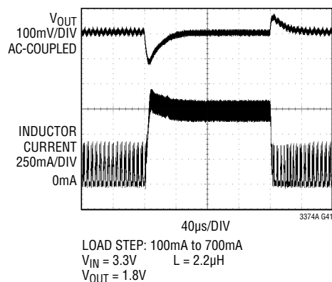
1A Buck Regulator, Transient Response (Burst Mode Operation)
