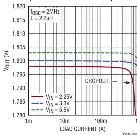
1A Buck Regulator Load Regulation (Forced Continuous Mode)
