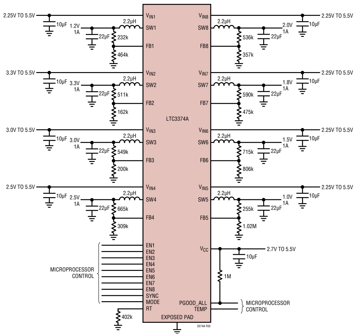
Figure 3. Detailed Front Page Application (All 1A Outputs)
