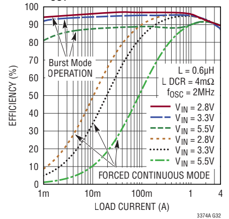
4A Buck Efficiency vs I_{\text{LOAD}} , V_{\text{OUT}} = 2.5\text{V}
