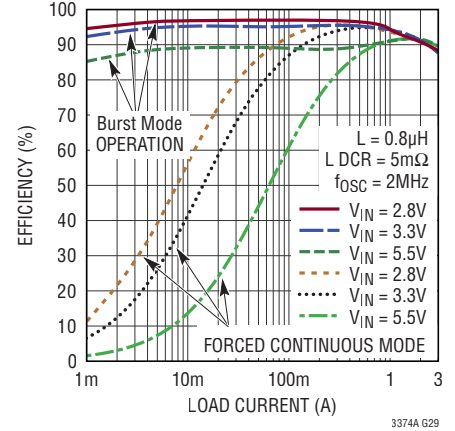
3A Buck Efficiency vs I_{\text{LOAD}} , V_{\text{OUT}} = 2.5\text{V}
