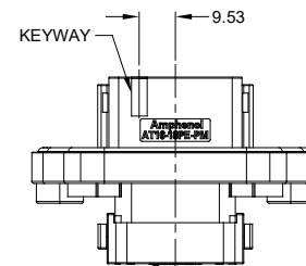
P/N AT16-18PE-PMXX KEY-E CONFIGURATION COLOR: GRAY
