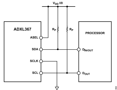
Figure 54. I 2 C Connection Diagram (Address 0x53)
