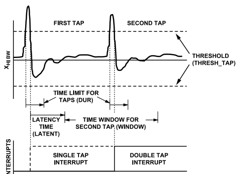
Figure 50. Tap Interrupt Function with Valid Single and Double Taps
