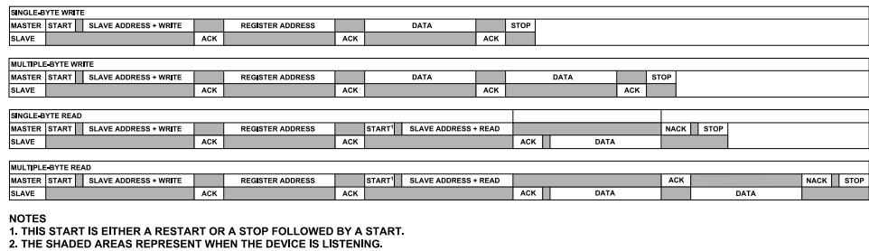
Figure 55. I 2 C Device Addressing (Read from Data Registers)
