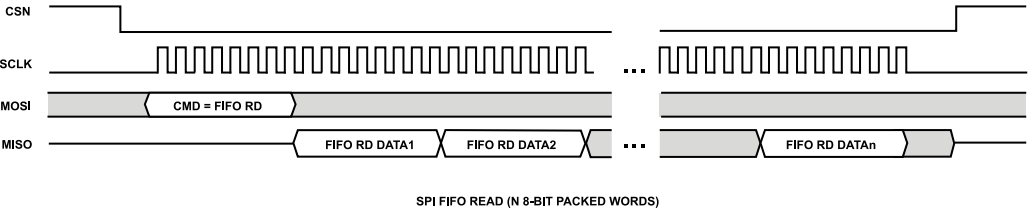
Figure 9. SPI FIFO Read (N 8-Bit Packed Words)
