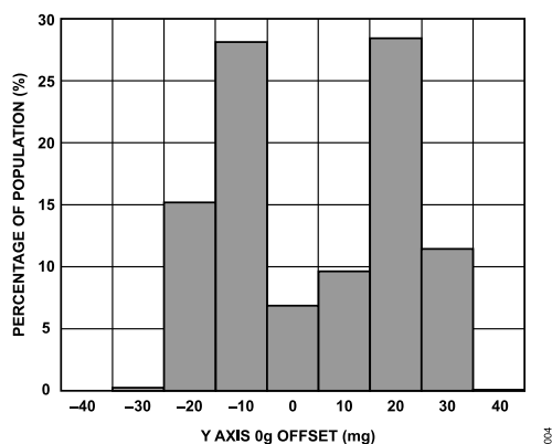
Figure 21. Y-Axis Zero g Offset at 25^\circ\text{C} , V_S = 2\text{ V}
