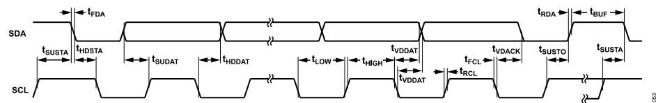
Figure 17. I²C Interface Timing Diagram
