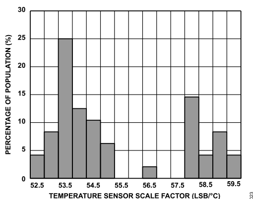
Figure 40. Temperature Sensor Scale Factor, V_S = 2\text{ V}
