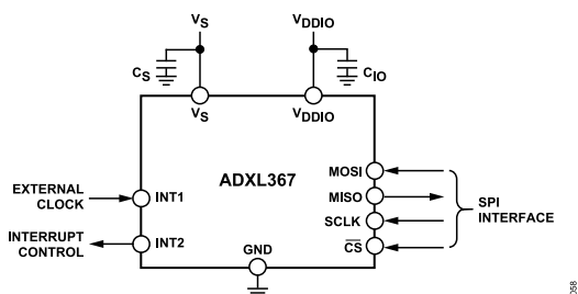
Figure 57. INT1 Pin as the Input for the External Clock
