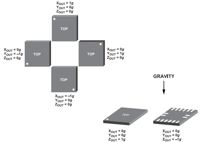
Figure 66. Output Response vs. Orientation to Gravity
