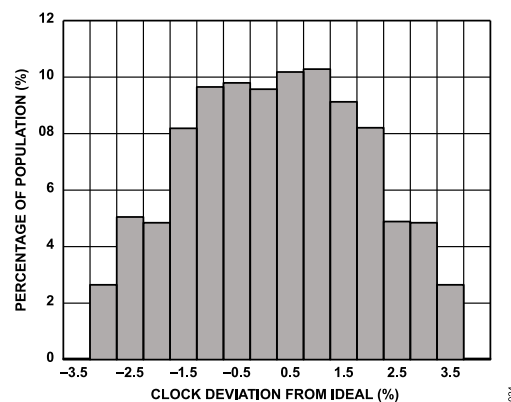
Figure 41. Clock Frequency Deviation from Ideal at 25°C, V_S = 2\text{ V}
