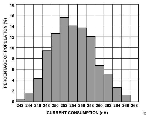
Figure 38. Current Consumption at 25°C, Wake-Up Mode, V_S = 2\text{ V}
