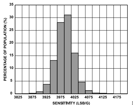
Figure 23. X-Axis Sensitivity at 25^\circ\text{C} , V_S = 2\text{ V} , \pm 2\text{ g} Range
