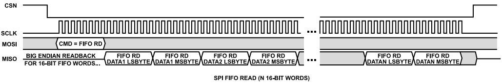
Figure 7. SPI FIFO Read (N 16-Bit Words)
