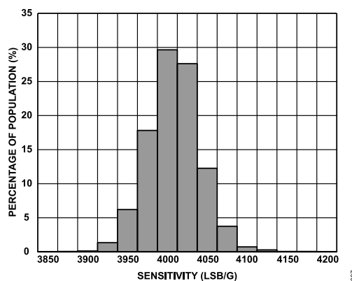
Figure 24. Y-Axis Sensitivity at 25^\circ\text{C} , V_S = 2\text{ V} , \pm 2\text{ g} Range
