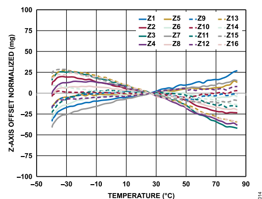
Figure 31. Z-Axis Offset Normalized vs. Temperature, 16 ADXL367 Devices Soldered to PCB, ODR = 100 Hz, V_S = 2\text{ V}
