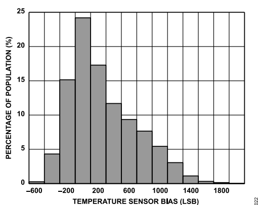
Figure 39. Temperature Sensor Response at 25°C, V_S = 2\text{ V}
