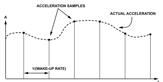
Figure 42. Acceleration Sampling
