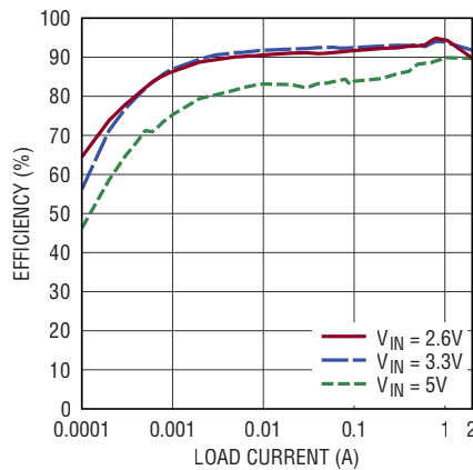
2.5V OUT Efficiency, 1MHz, Burst Mode Operation
