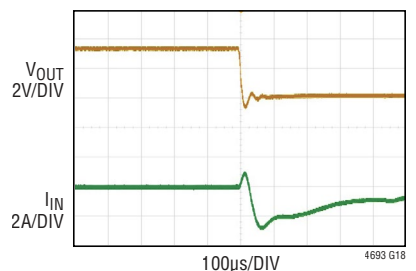
Short-Circuit with 2A Load
