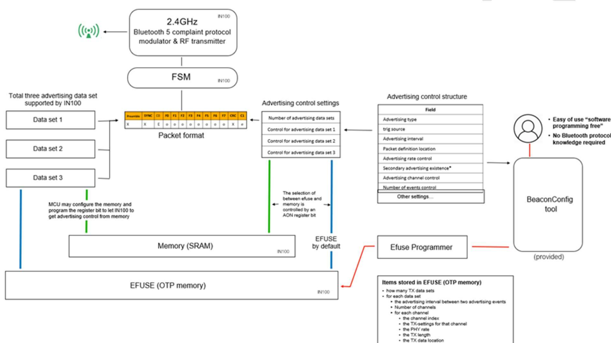
Figure 4 : Advertising packet and advertising packet creation process overview
