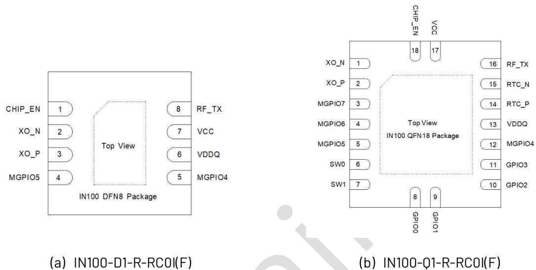
Figure 3 : Pin assignments
