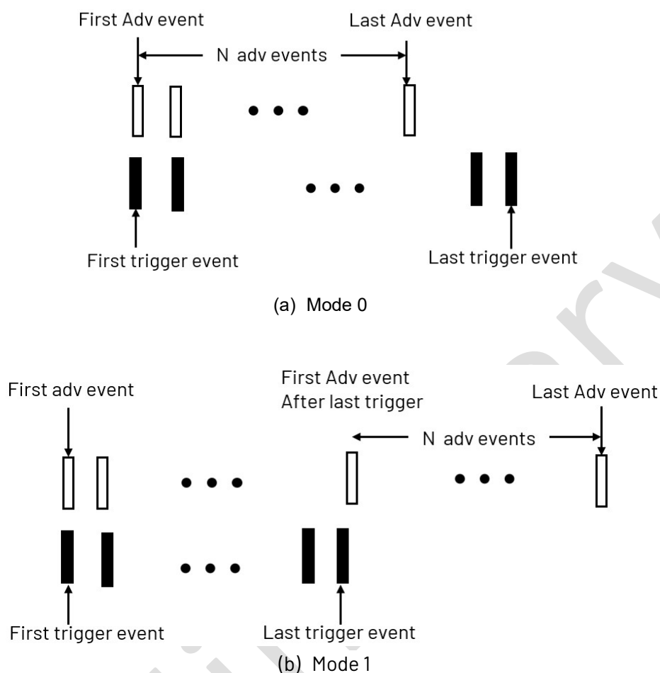
Figure 5 : Trigger modes
