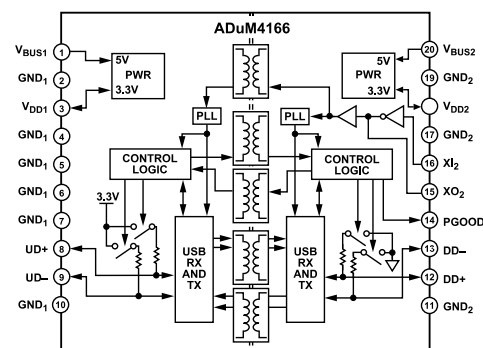
Figure 2. ADuM4166 Clock Input from Peripheral Side
