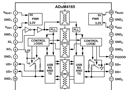
Figure 1. ADuM4165 Clock Input from Host Side
