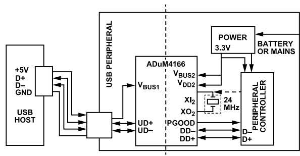
Figure 18. ADuM4166 Isolated USB Peripheral Application
