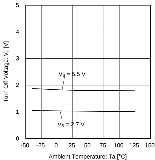
Figure 44. Turn Off Voltage vs Ambient Temperature
