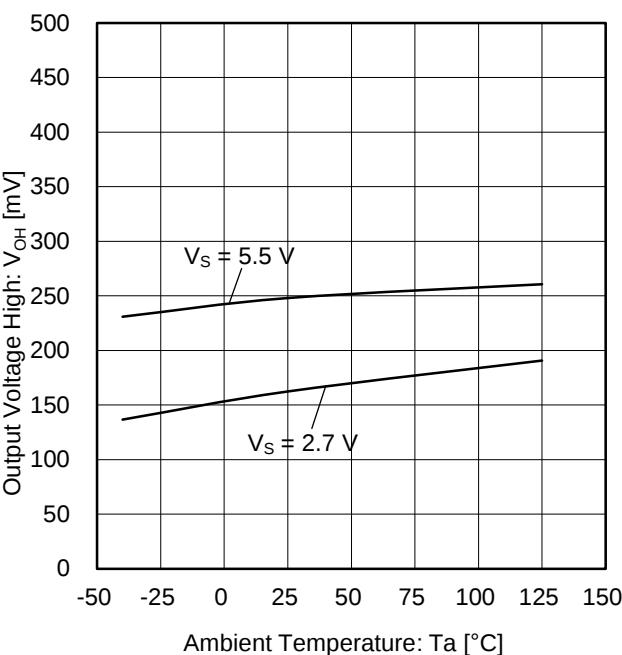
Figure 4. Output Voltage High vs Ambient Temperature ( R_L = 100\ \Omega , V_{OH} = V_{DD} - V_{OUT} )
