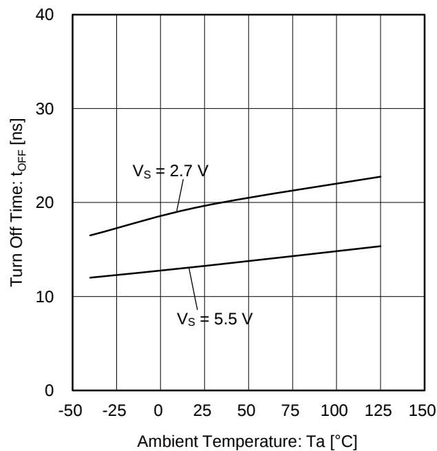
Figure 42. Turn Off Time vs Ambient Temperature
