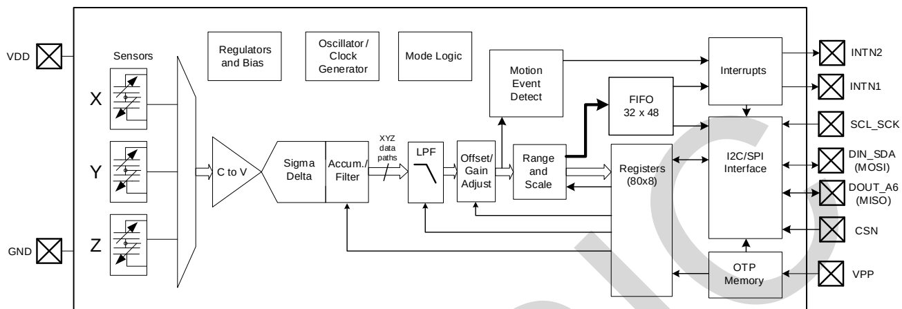
Figure 1. Block Diagram
