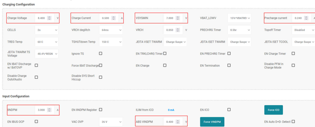
Figure 2-7. Charger Configuration
