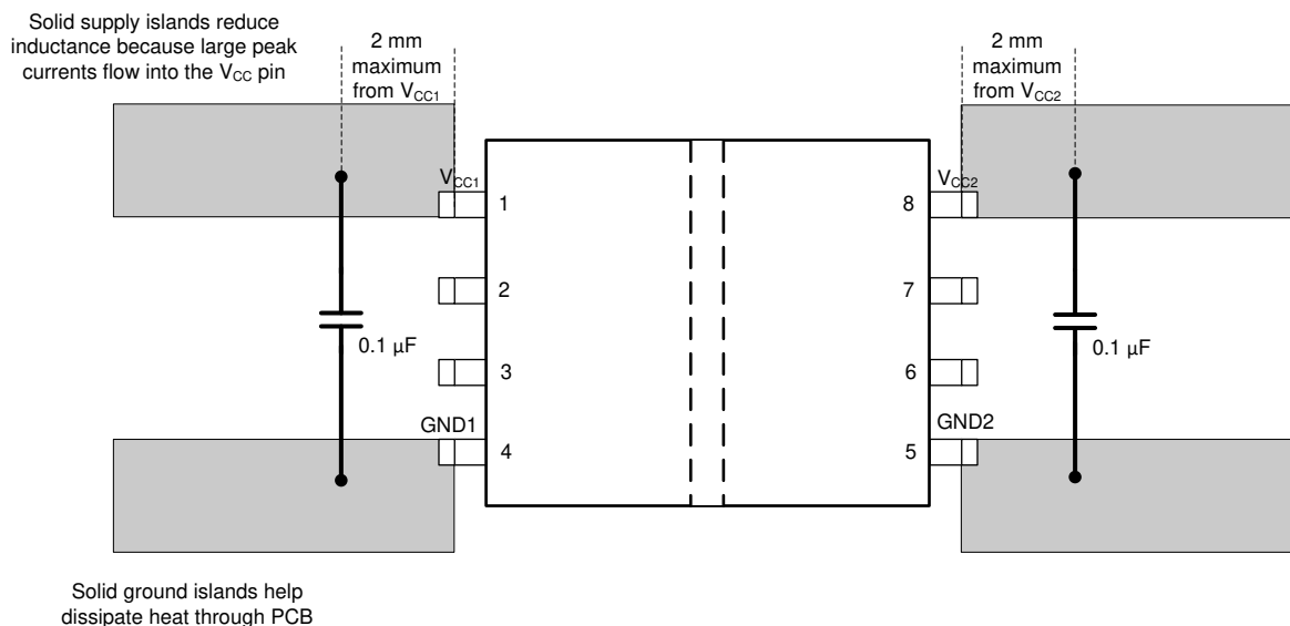
Figure 12-1. Layout Example
