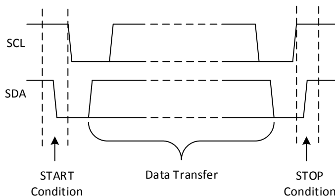
Figure 8-4. Definition of Start and Stop Conditions
