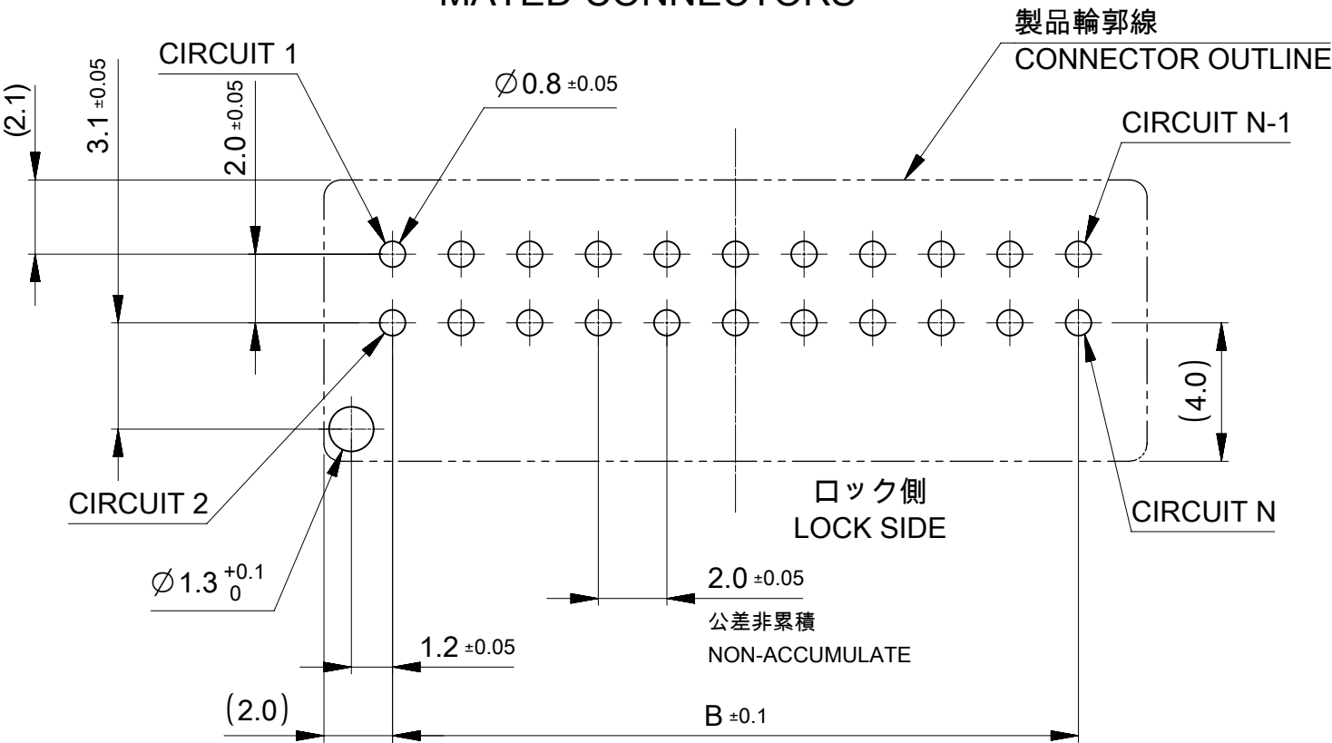
基板取付穴推奨寸法(マウント面) POLARIZED RECOMMENDED PCB LAYOUT HOLE DIMENSION (MOUNTING SIDE) 参考基板厚 t=1.2~1.6 REFERENCE PCB THICKNESS t=1.2~1.6
