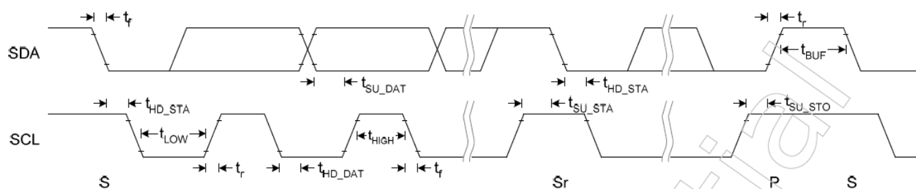
Figure 7 I2C Fast Mode Timing
