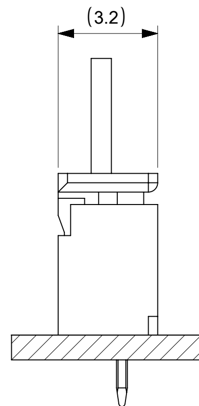
1 嵌合図 MATED CONNECTORES
