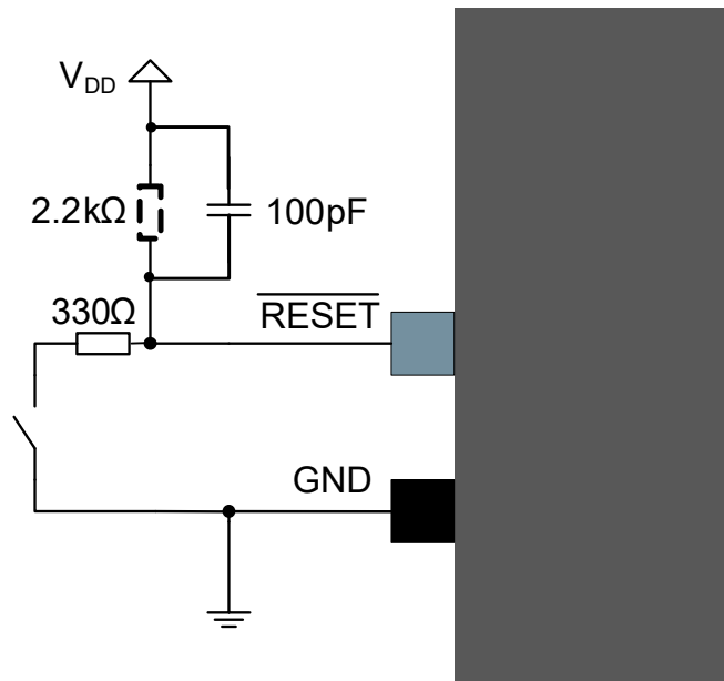
Figure 53-6. External Reset Circuit Schematic (EFT Immunity Enhancement)
