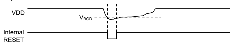
Figure 45-2. BODVDD Hysteresis OFF
