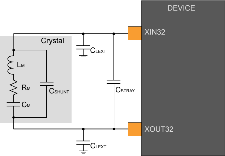
Figure 49-5. Oscillator Connection
