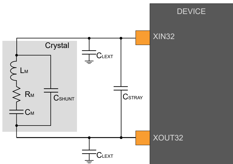
Figure 45-6. Oscillator Connection
