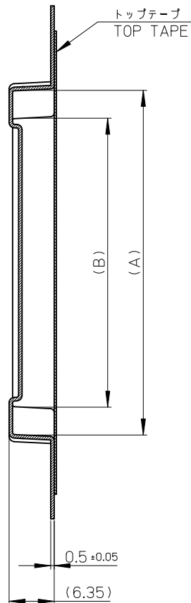
SECT. Y-Y
