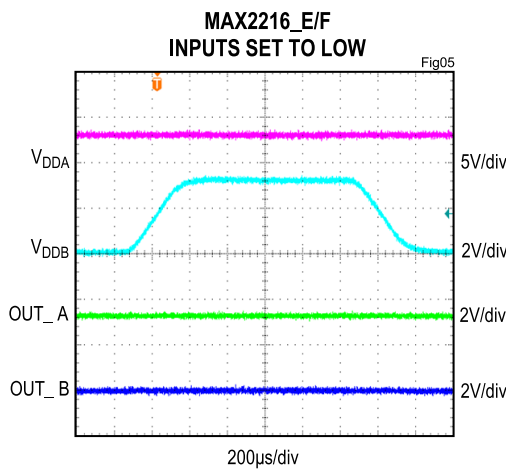
Figure 5. Undervoltage Lockout Behavior, MAX2216_E/F, Inputs Set to Low
