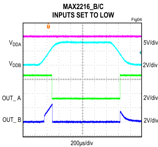
Figure 4. Undervoltage Lockout Behavior, MAX2216_B/C, Inputs Set to Low
