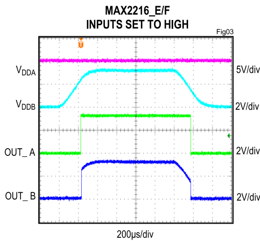
Figure 3. Undervoltage Lockout Behavior, MAX2216_E/F, Inputs Set to High
