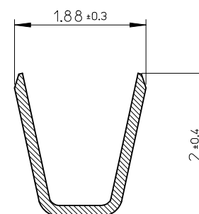
SECTION Y-Y SCALE 20:1
