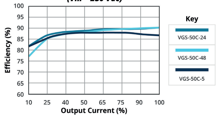
EFFICIENCY VS OUTPUT LOAD ( V_{in} = 230 \text{ Vac} )
