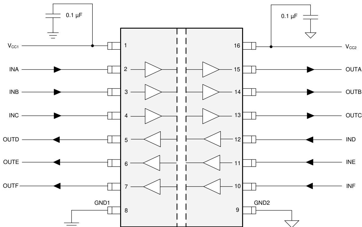
Figure 9-2. Typical ISO676x Circuit Hook-up
