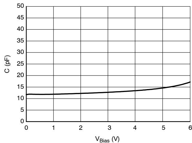
Figure 3. CV Characteristics
