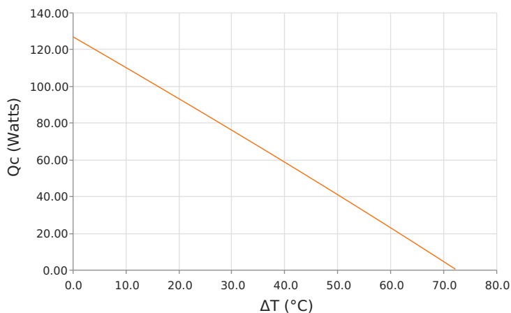
Heat Pumped at Cold Side ( Q_c ) T_{hot} = 27\text{ }^{\circ}\text{C} | Current = 13.2 Amps
