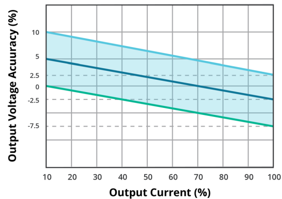
OUTPUT REGULATION CURVE 5 Vdc input / all other output models (nominal input)
