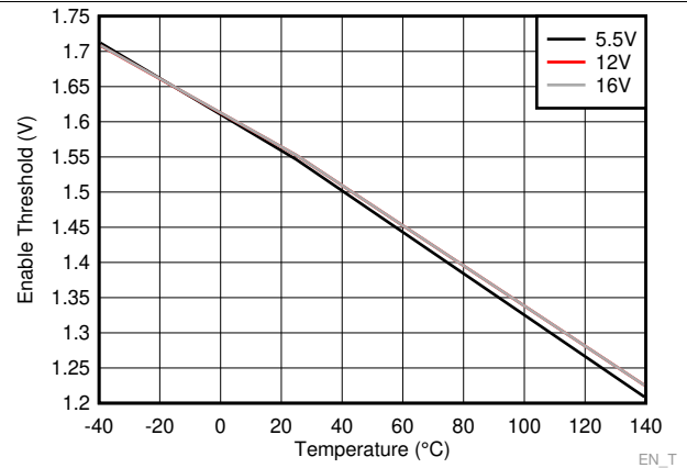
Figure 10. Enable Threshold
