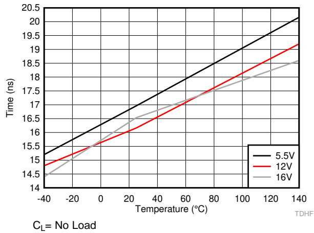
Figure 29. HO Falling Propagation Delay (TDHF)
