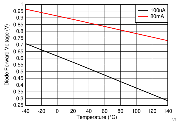
Figure 16. Boot Diode Forward Voltage Drop
