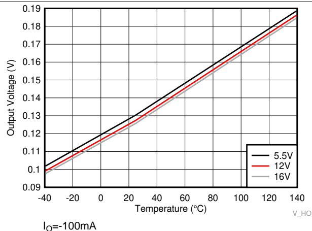
Figure 21. HO High Output Voltage ( V_{HOH} )
