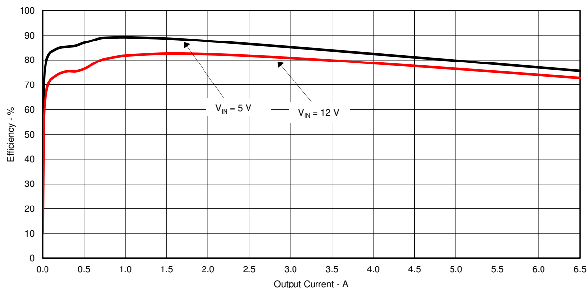
Figure 4-1. TPS54626EVM-608 Efficiency
