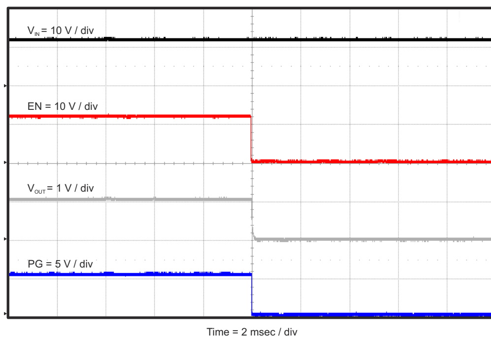
Figure 4-14. TPS54626EVM-608 Shut-Down Relative to EN
