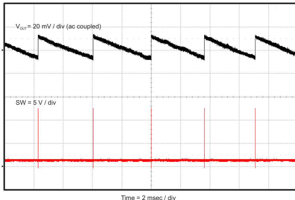
Figure 4-9. TPS54626EVM-608 Output Voltage Ripple, I_{OUT} = 10 mA
