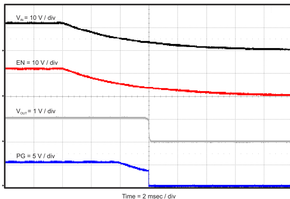
Figure 4-13. TPS54626EVM-608 Shut-Down Relative to V_{IN}
