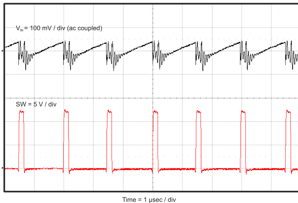
Figure 4-10. TPS54626EVM-608 Input Voltage Ripple, I_{OUT} = 6.5 A
