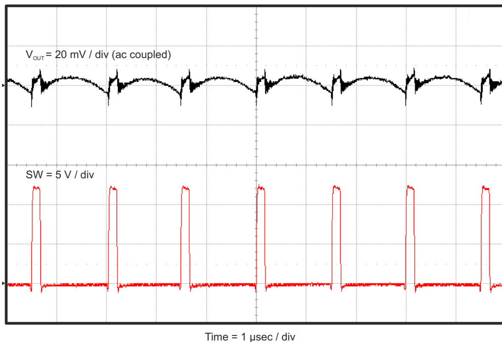
Figure 4-7. TPS54626EVM-608 Output Voltage Ripple, I_{OUT} = 6.5 A
