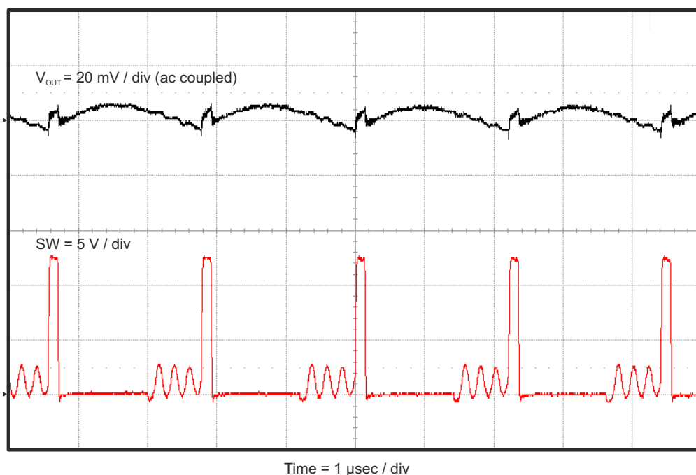
Figure 4-8. TPS54626EVM-608 Output Voltage Ripple, I_{OUT} = 300 mA
