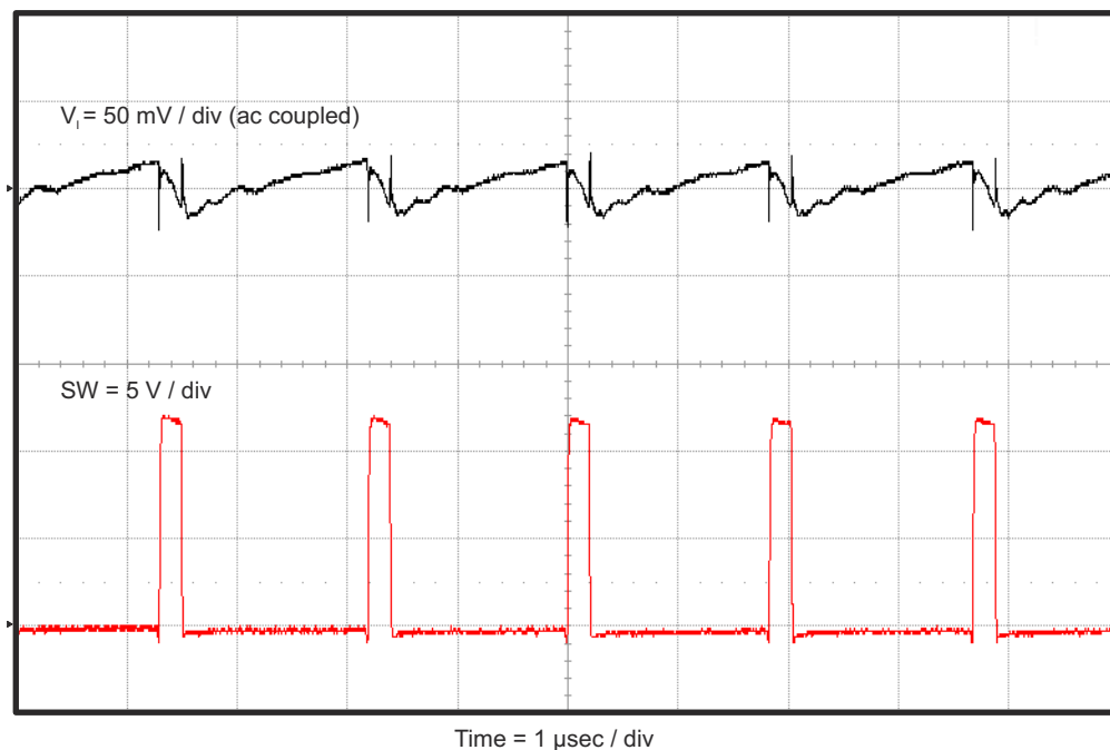
Figure 4-8. TPS563219AEVM-663 Input Voltage Ripple, I_{OUT} = 3 A
