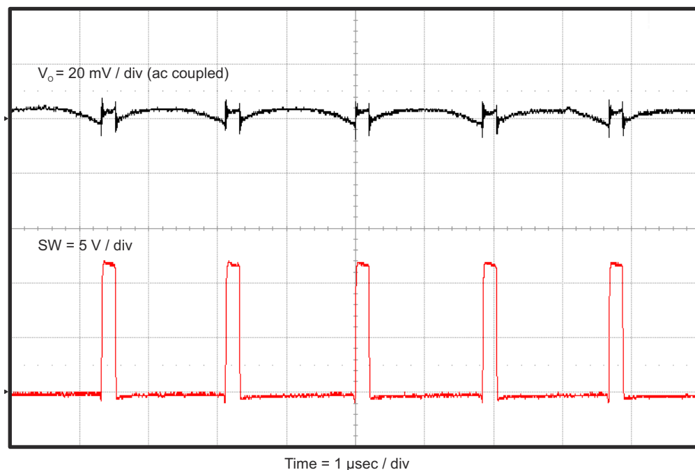
Figure 4-7. TPS563219AEVM-663 Output Voltage Ripple, I_{OUT} = 3 A
