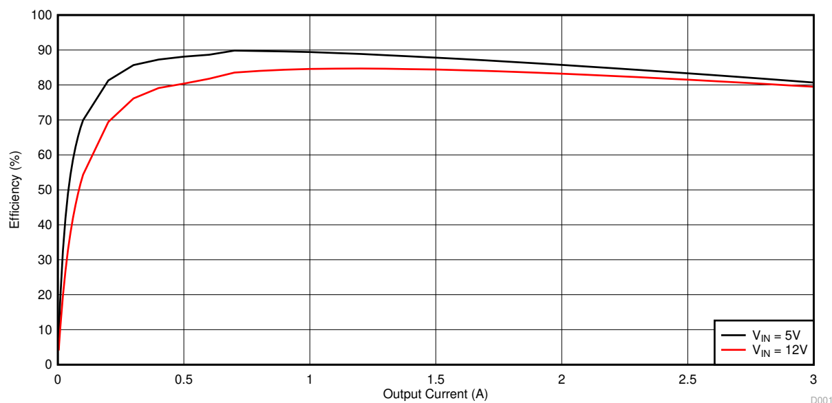
Figure 4-1. TPS563219AEVM-663 Efficiency
