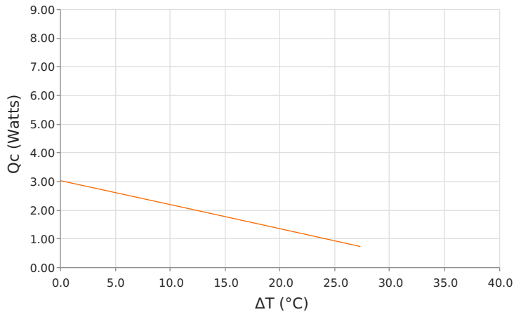
Heat Pumped at Cold Side ( Q_c ) T_{hot} = 85\text{ }^{\circ}\text{C} | Current = 2.6 Amps
