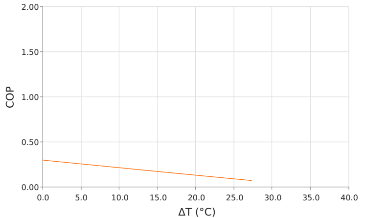
Coefficient of Performance (COP = Q_c/P_{in} ) T_{hot} = 85\text{ }^{\circ}\text{C} | Current = 2.6 Amps
