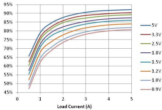
Figure 4. Efficiency vs. Output Voltage, I_{out}=5A , F_{sw}=500kHz
