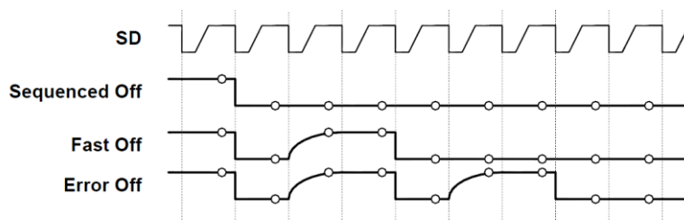
Figure 40. OK Severity Encoding Waveforms
