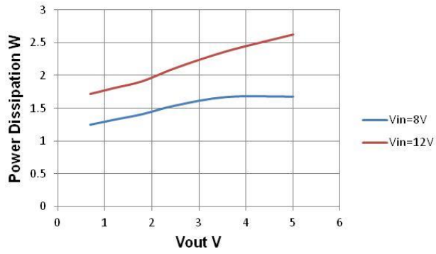
Figure 10. Power Dissipation vs Vout, Iout=5A, Fsw=1MHz
