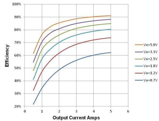
Figure 6. Efficiency vs. Load, V_{in}=12V , F_{sw}=1MHz
