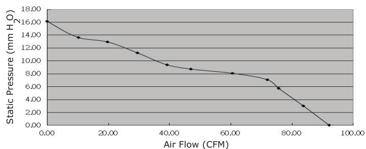
CFM-9238S-250-532
