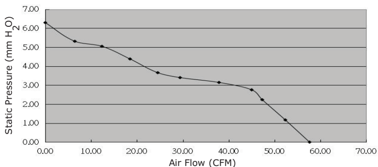
CFM-9238S-230-410
