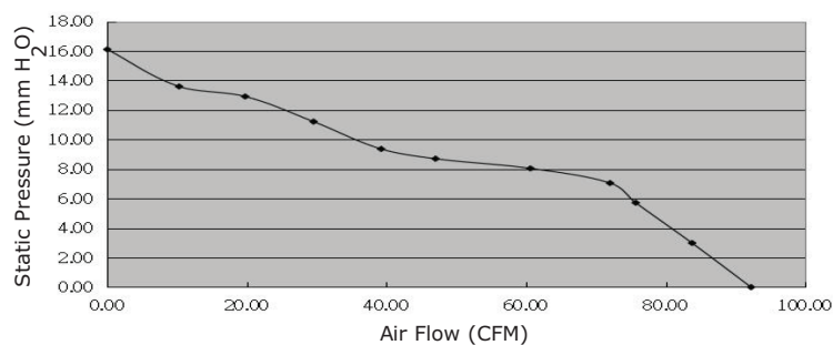
CFM-9238S-148-523
