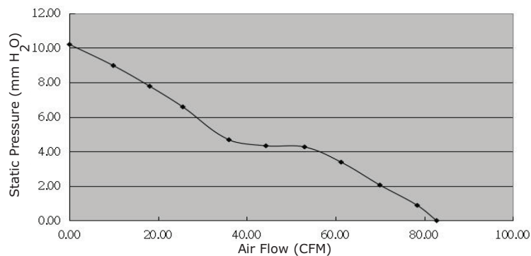
CFM-9238S-250-532
