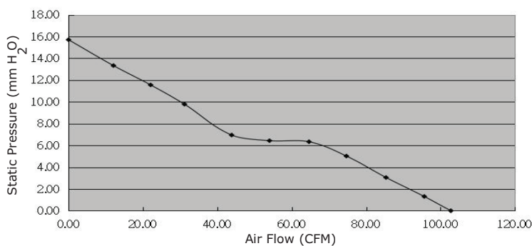
CFM-9232S-250-509
