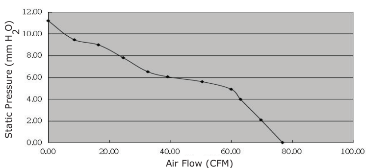
CFM-9238S-240-473
