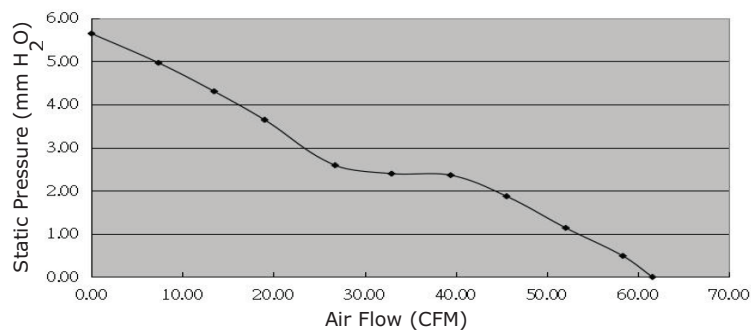
CFM-9232S-230-398
