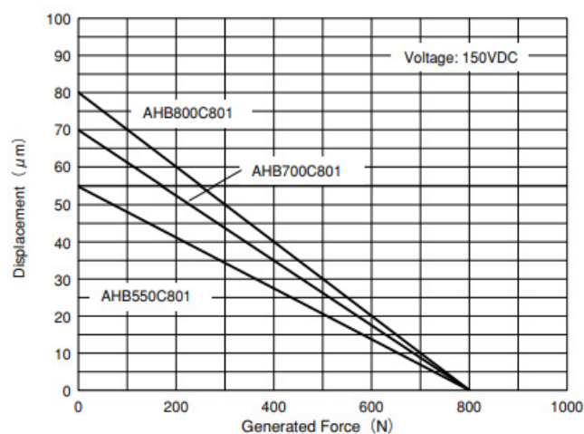
Figure 2 - Compression Load vs. Displacement
