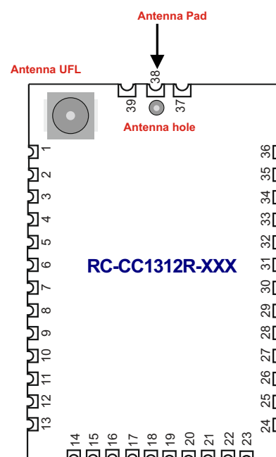
Pin out device
