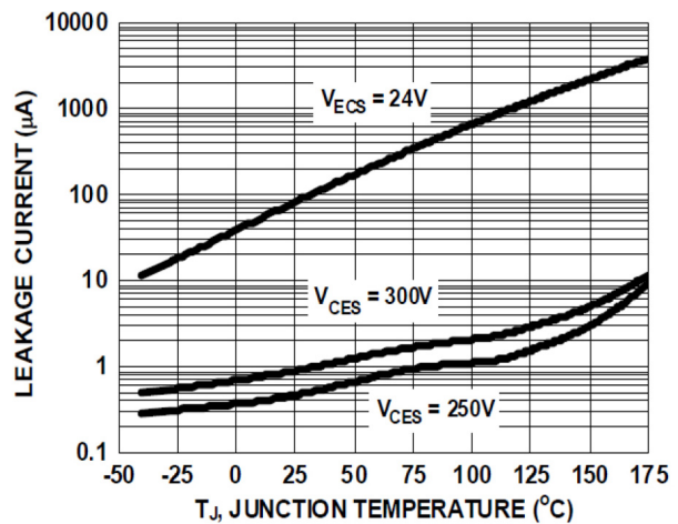
Figure 12. Leakage Current vs. Junction Temperature
