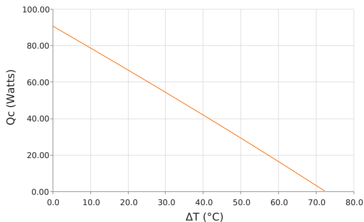
Heat Pumped at Cold Side ( Q_c ) T_{hot} = 27\text{ }^{\circ}\text{C} | Current = 9.5 Amps
