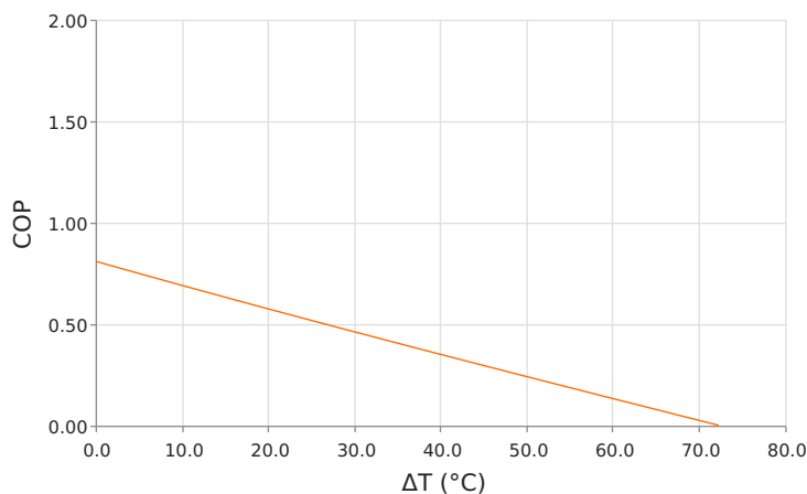
Coefficient of Performance (COP = Q_c/P_{in} ) T_{hot} = 27\text{ }^{\circ}\text{C} | Current = 9.5 Amps
