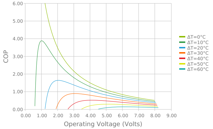
Coefficient of Performance (COP = Q_c/P_{in} ) T_{hot} = 27^\circ\text{C}
