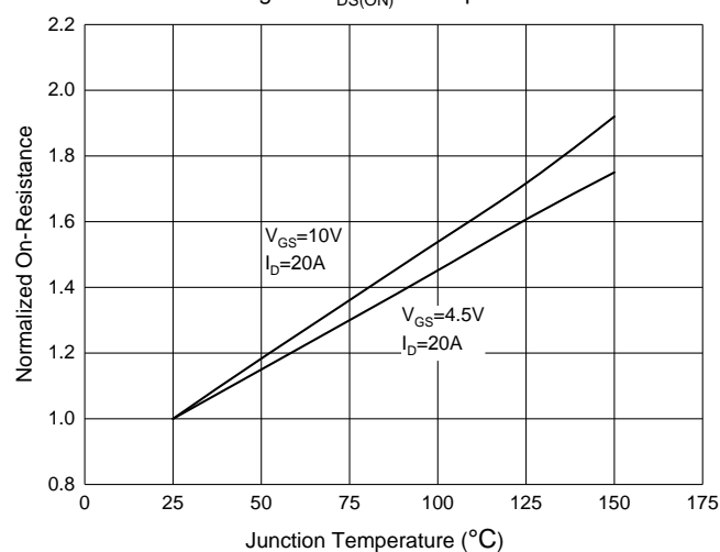
Fig. 6 - R_{DS(ON)} - \text{Temperature}
