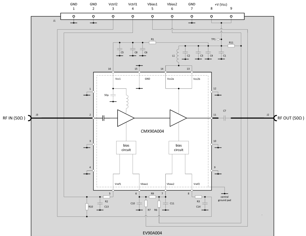
Figure 30: EV90A004 Schematic
