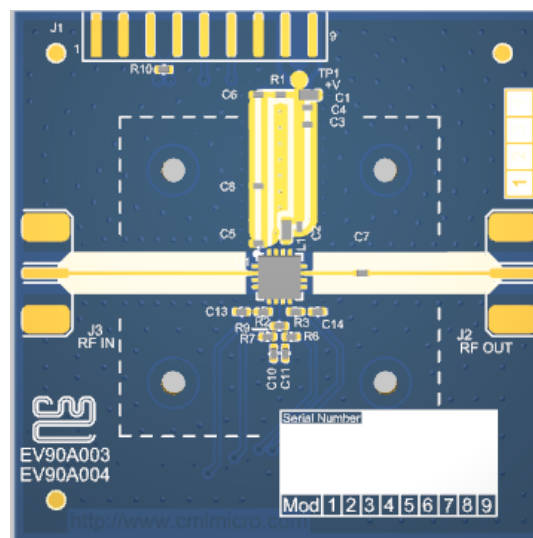
Figure 32: EV90A004 PCB Top Layer View
